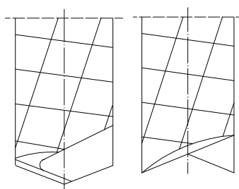
Bohrspitzen- anschliff drill point cut
