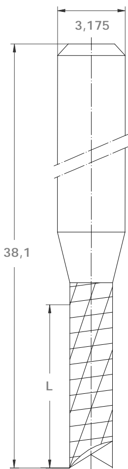
Bohrspitzen- anschliff drill point cut
