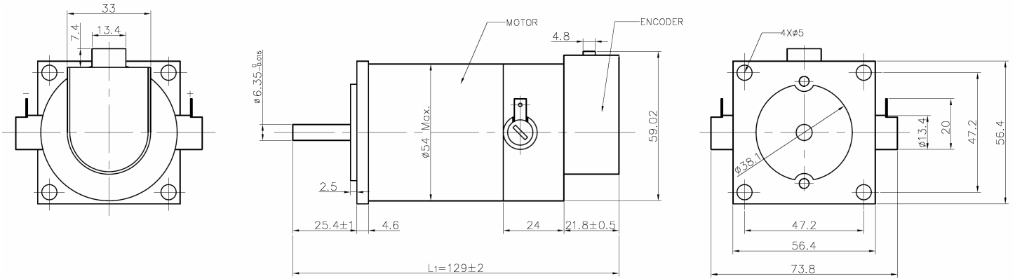
Figure 1: Mechanical specification of DCM57202 motor (plus encoder)
