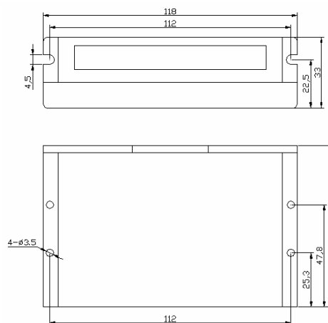
Figure 1: Mechanical specifications
