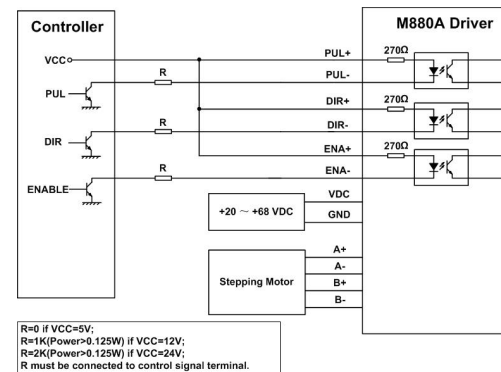
Figure 10: Typical connection
